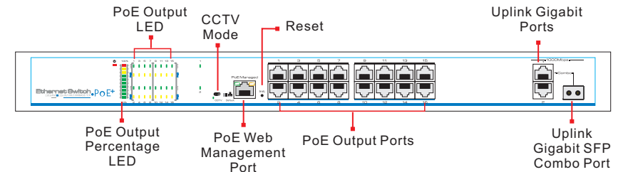
16 Ports PoE switch
